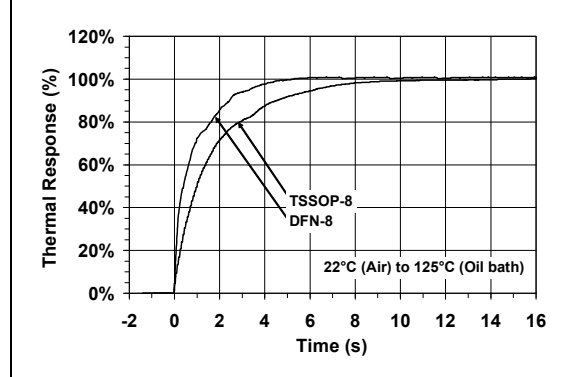
FIGURE 2-12: Package Thermal Response.
