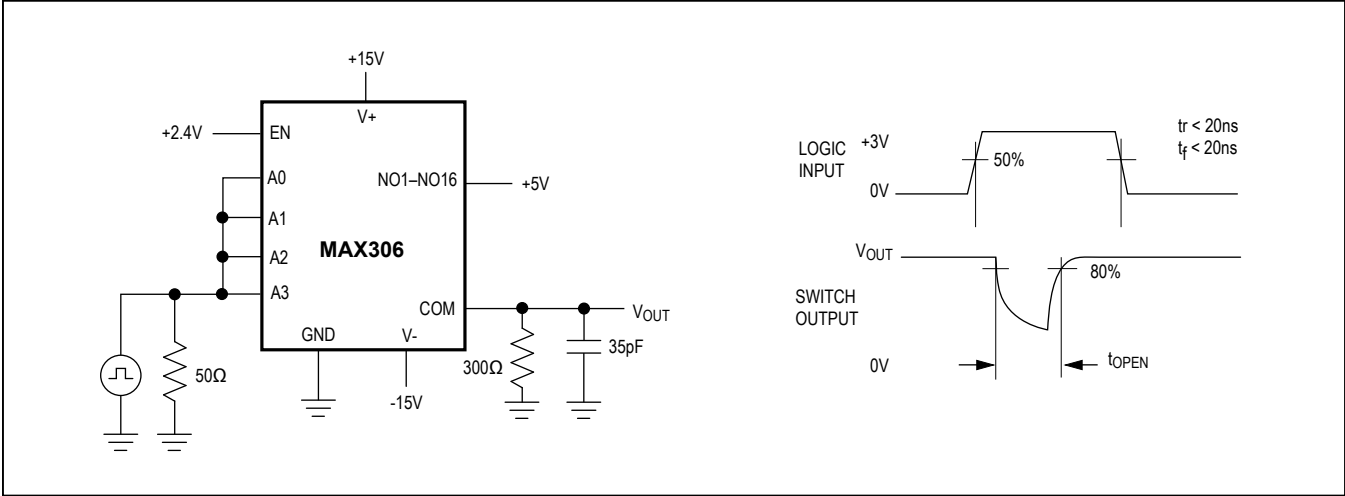
Figure 4. Break-Before-Make Interval
