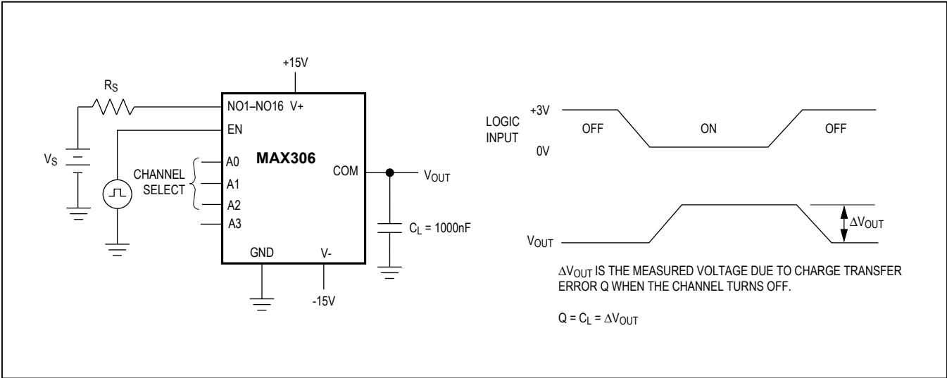
Figure 5. Charge Injection
