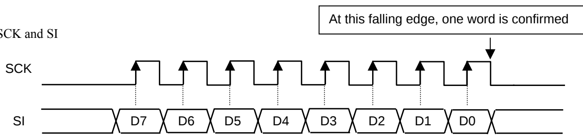
Timing of Serial Data Transfer
