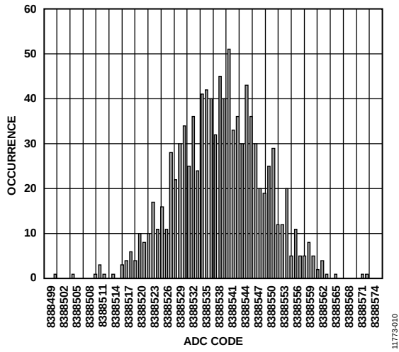
Figure 10. Noise Distribution Histogram (Output Data Rate = 10 kSPS, Analog Input Buffers Disabled)
