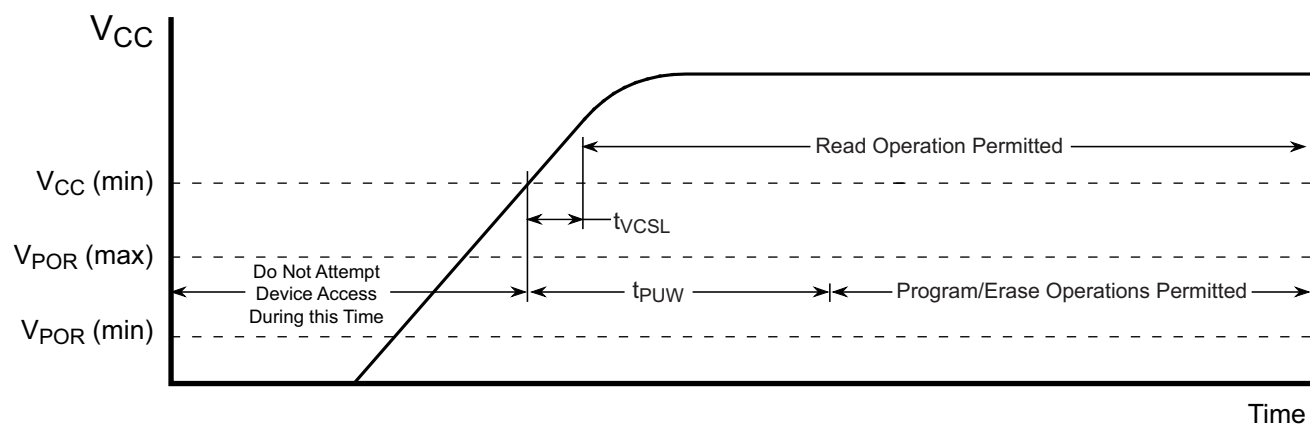
Figure 16-1. Power-Up Timing
