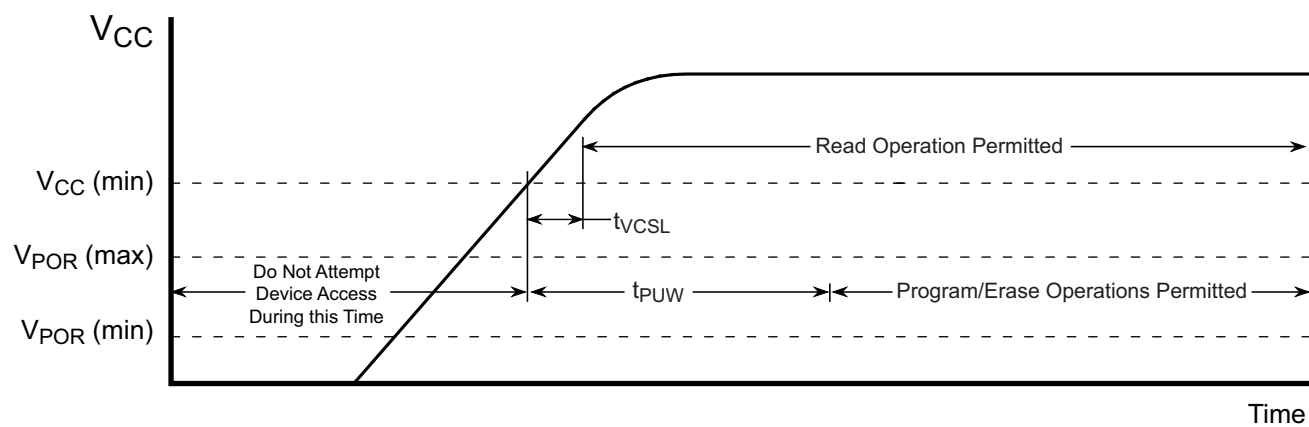
Figure 16-1. Power-Up Timing
