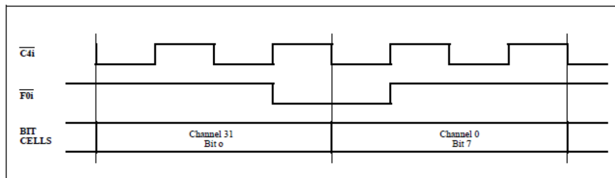
Figure 12 - Frame Alignment
