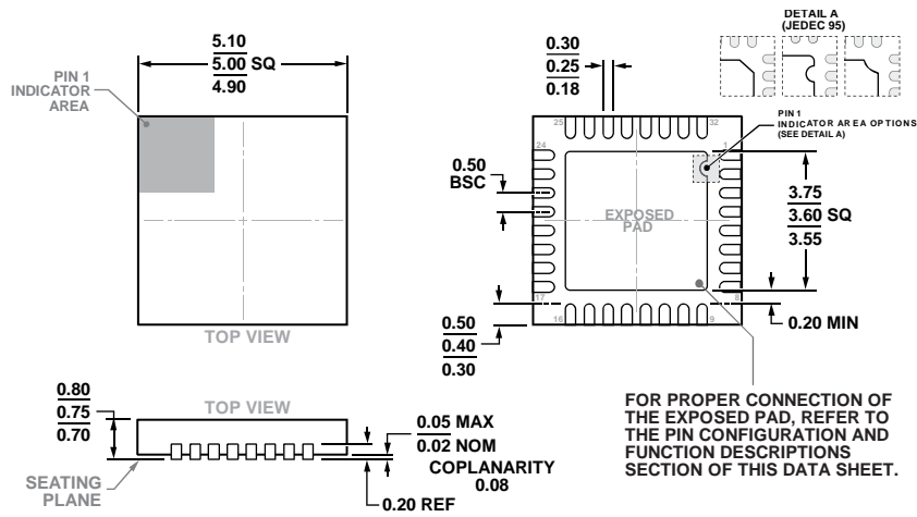
COMPLIANT TO JEDEC STANDARDS MO-220-WHHD-5 Figure 25. 32-Lead Lead Frame Chip Scale Package [LFCS] 5 mm × 5 mm Body and 0.75 mm Package Height (CP-32-12) Dimensions shown in millimeters
