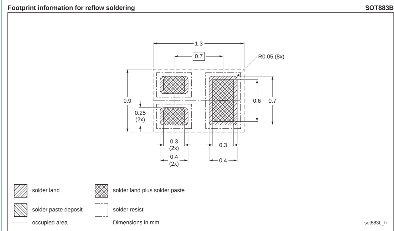
Fig 11. Reflow soldering footprint for SOT883B
