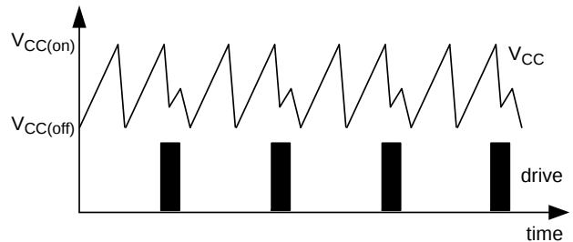
Figure 44. Auto-Recovery Double Hiccup Sequence
