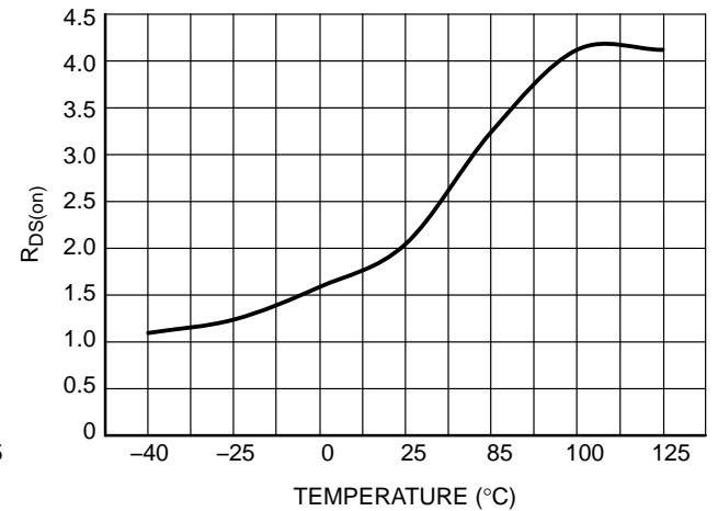
Figure 32. NCP 1129 R_{DS(on)} vs. Junction Temperature
