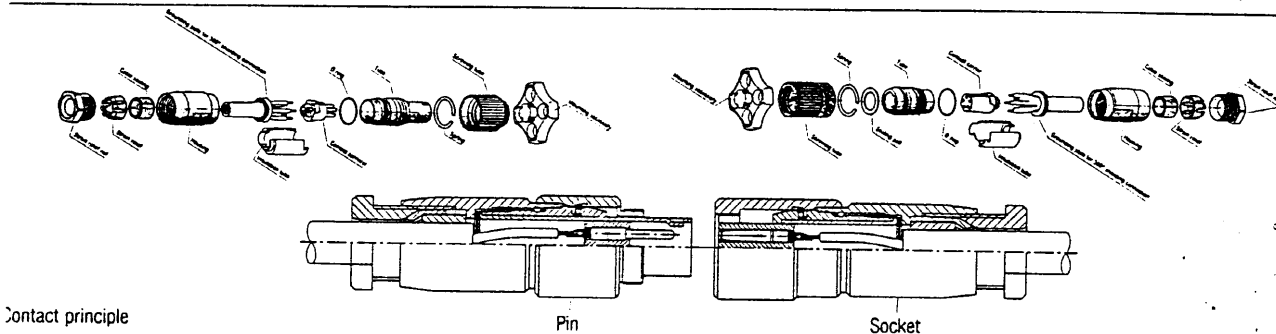
Arrangement of Contacts
