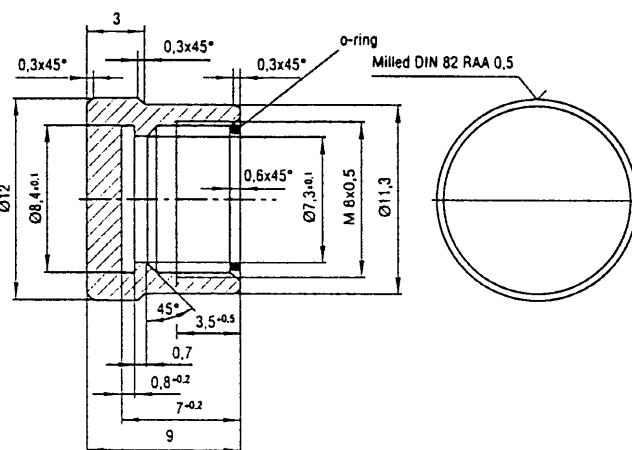
Dust cap: for pin connectors
