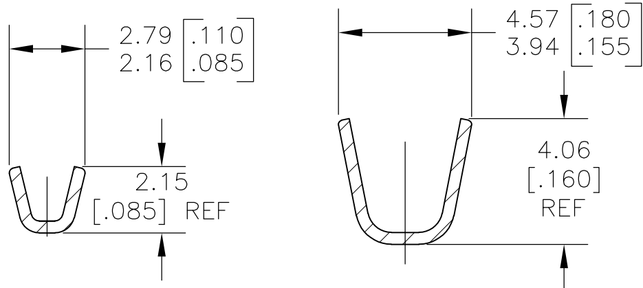
SECTION A-A SECTION B-B
