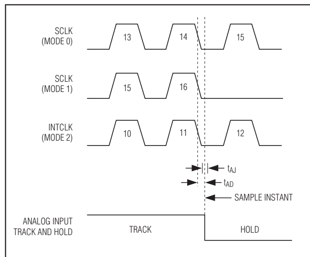
Figure 19. Aperture Diagram
