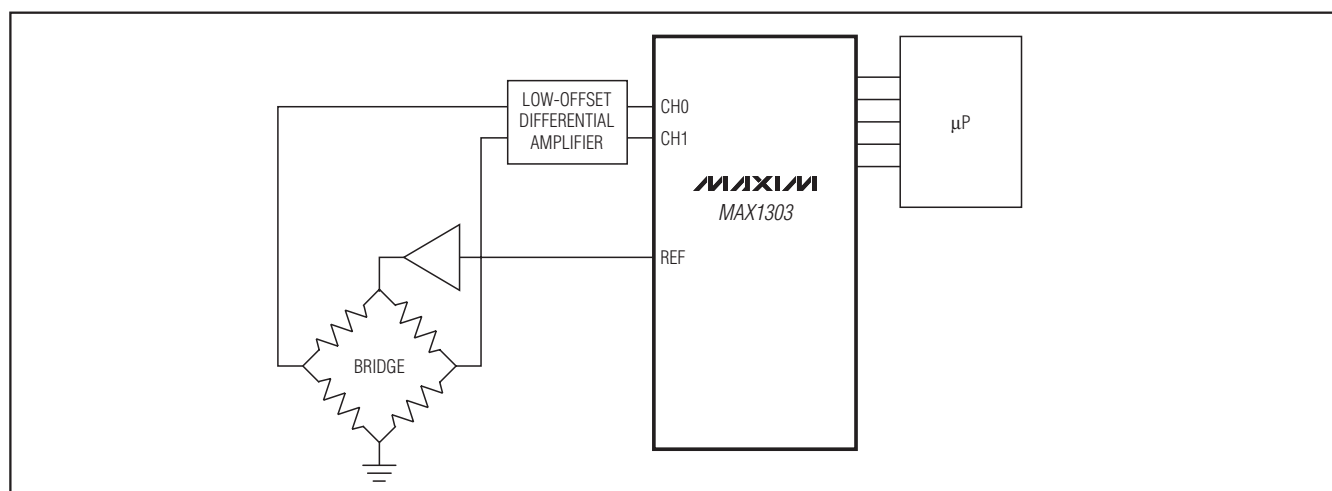
Figure 18. Bridge Application
