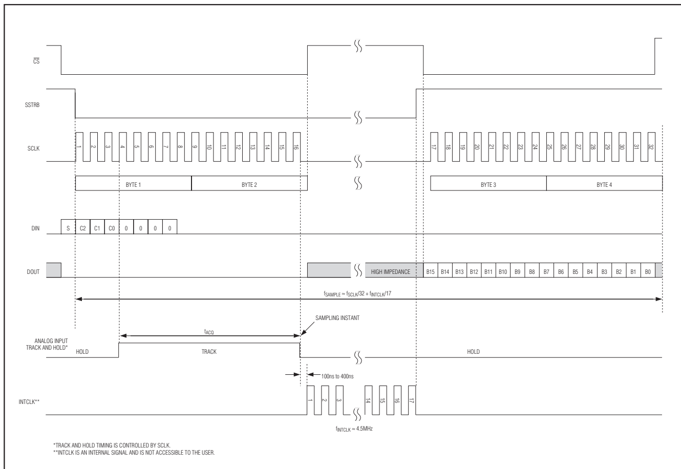
Figure 2. External Acquisition-Mode Conversion (Mode 1)
