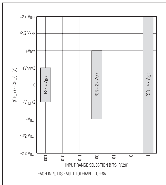
Figure 7. Differential Input Voltage Ranges
