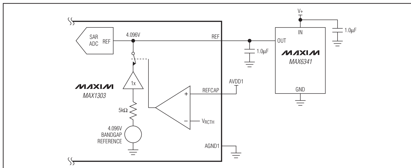
Figure 17. External Reference Operation
