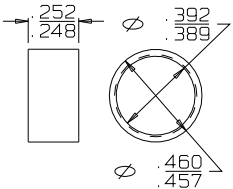
SCREW TJSS-106-3
