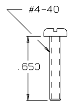
SCREW TJSS-106-19
