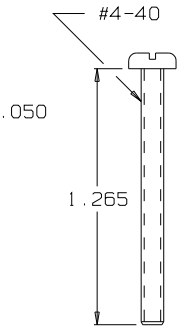
SCREW TJSS-106-3
