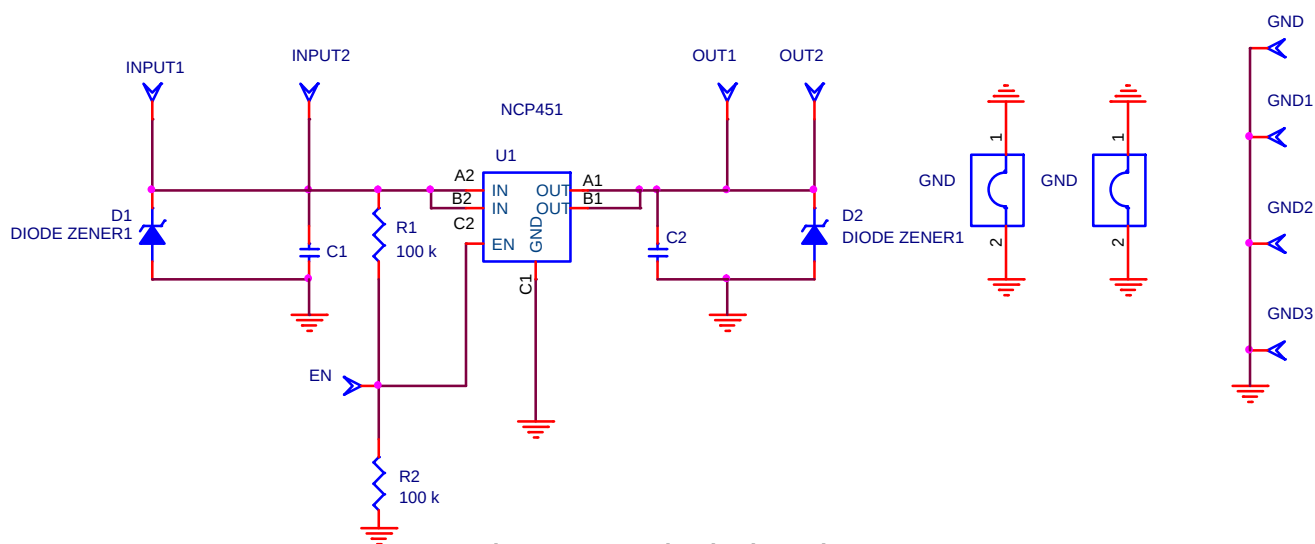
Figure 14. Demobard schematic
