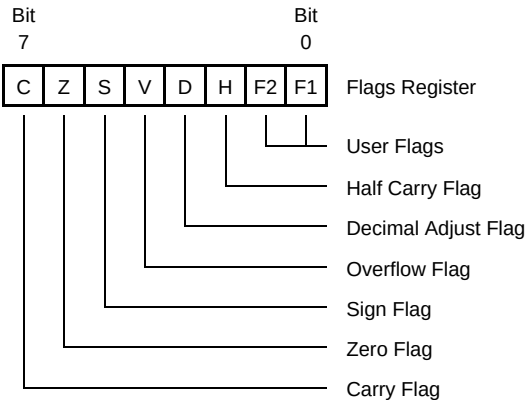
Figure 56. Flags Register
