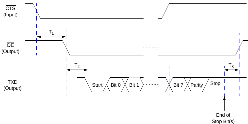
Figure 54. UART Timing with \overline{CTS}
