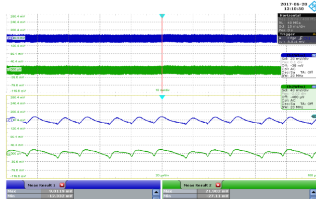
Figure 53 – Output Ripple Voltage Waveforms. 265 VAC Input. 5 V PK : 22 mV, 12 V PK : 50 mV. Upper: 5 V, 20 mV / div. Lower: 12 V, 40 mV / , 10 ms, 20 \mu s / div.
