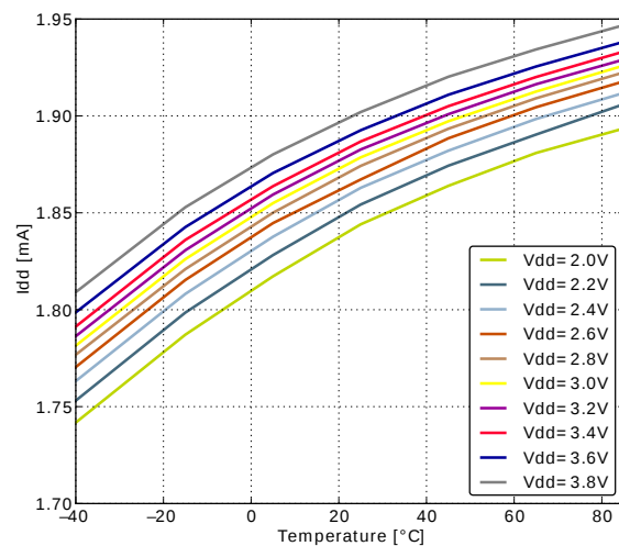
Figure 3.8. EM1 Current consumption with all peripheral clocks disabled and HFRCO running at 28MHz
