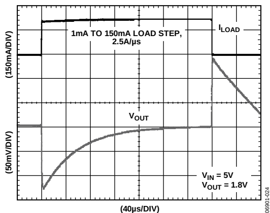
Figure 23. Load Transient Response, C_{IN} = C_{OUT} = 1\ \mu\text{F}
