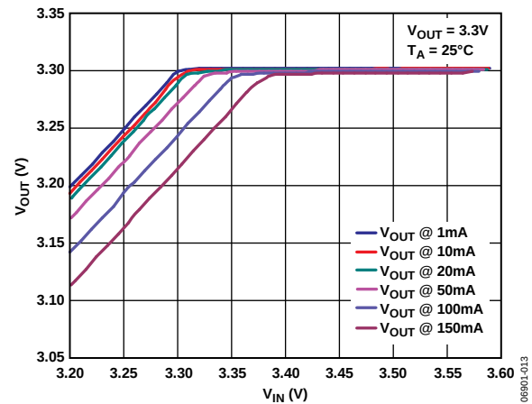
Figure 15. Output Voltage vs. Input Voltage (In Dropout), WLCS
