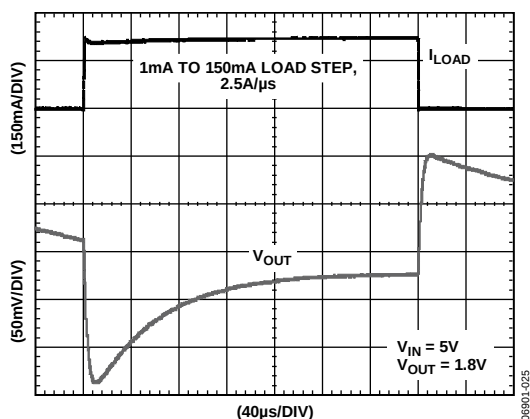
Figure 24. Load Transient Response, C_{IN} = C_{OUT} = 4.7\ \mu\text{F}
