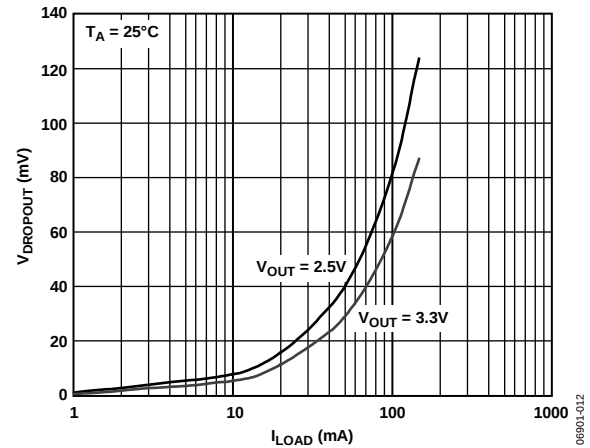
Figure 14. Dropout Voltage vs. Load Current, WLCS
