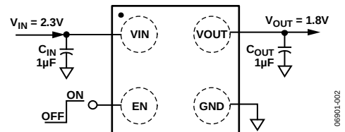
Figure 2. ADP121 WLCSP with Fixed Output Voltage, 1.8 V
