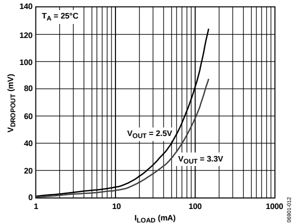
Figure 14. Dropout Voltage vs. Load Current, WLCSP
