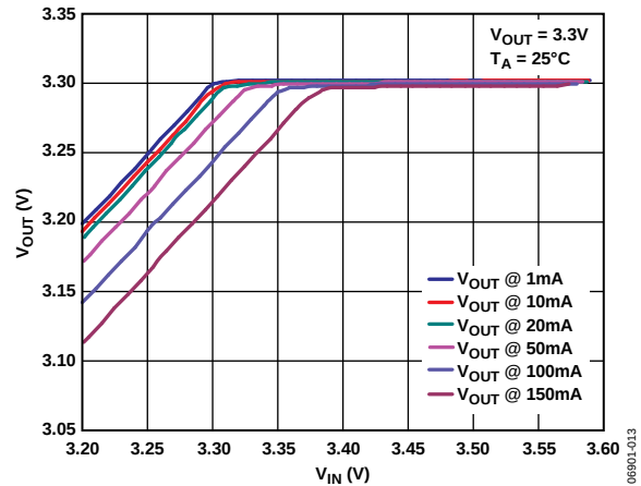
Figure 15. Output Voltage vs. Input Voltage (In Dropout), WLCSP
