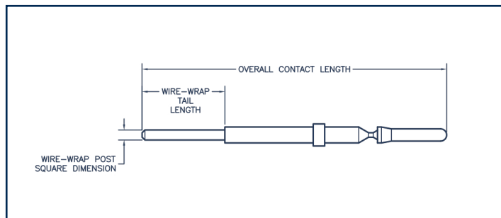
Wire-Wrap Contact
