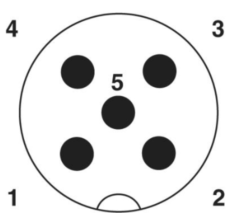
Male/Female M12
