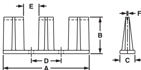
High Holder (FSHH-X)
