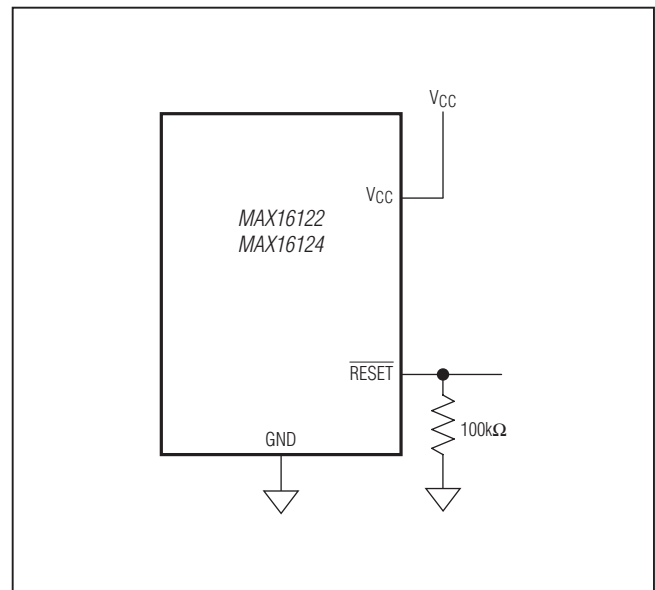
Figure 2. Ensuring \overline{RESET} Output to V_{CC} = 0V
