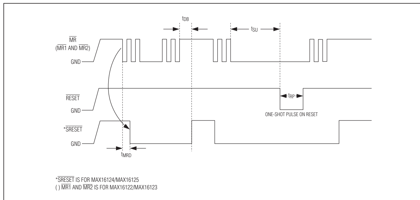
Figure 1a. Reset Timing Diagram
