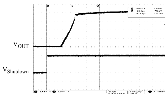
Figure 36. Soft Start Time (Conditions: I_{OUT}=0\text{mA} , C_{IN}=C_{OUT}=1\mu\text{F} , V_{Shutdown}=0 to 2\text{V} , V_{OUT}=0.8\text{V} )
