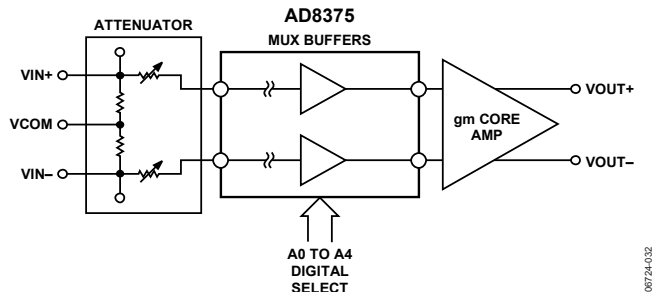
Figure 32. Simplified Schematic
