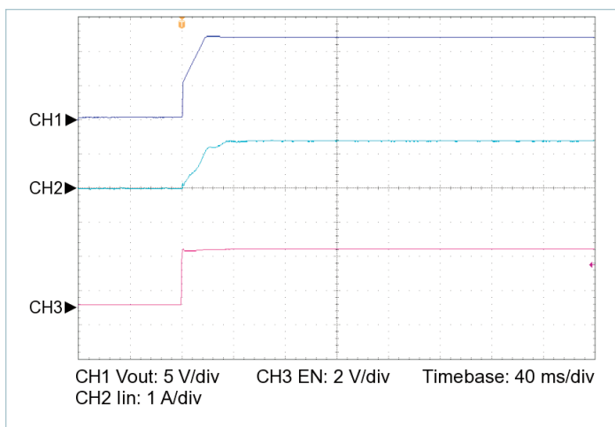
Figure 17 — Startup from EN, V_{IN} = 300\text{ V} , C_{OUT\_EXT} = 10000\text{ μF} , R_{LOAD} = 0.359\text{ Ω}
