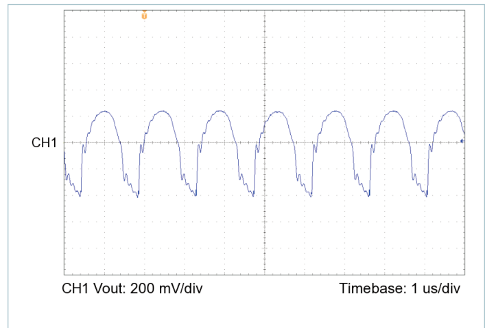
Figure 19 — Output voltage ripple, V_{IN} = 300\text{ V} , V_{OUT} = 12.0\text{ V} , C_{OUT\_EXT} = 1000\text{ μF} , R_{LOAD} = 0.359\text{ Ω}
