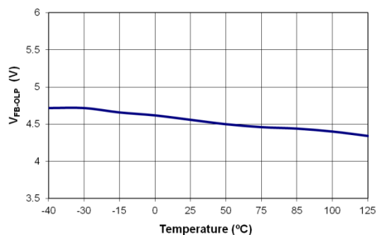
Figure 17. FB Open-Loop Trigger Level ( V_{FB-OLP} ) vs. Temperature
