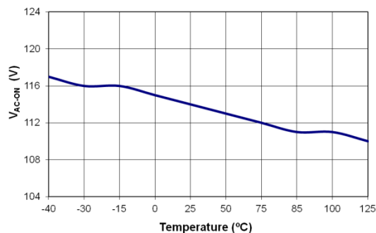
Figure 23. Brown-In ( V_{AC-ON} ) vs. Temperature
