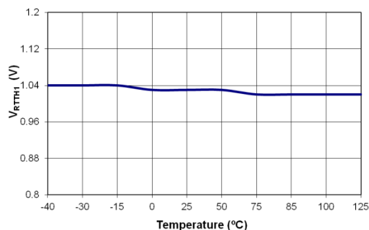
Figure 21. Over-Temperature Protection Threshold Voltage ( V_{RTTH1} ) vs. Temperature
