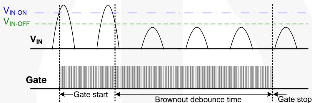
Figure 6. Brownout Behavior
