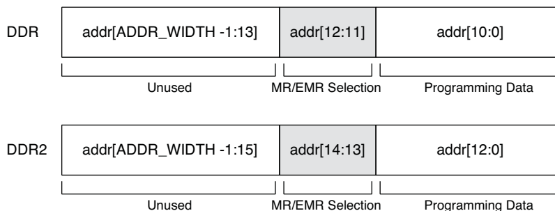
Figure 2-9. Local-to-Memory Address Mapping for MR/EMR Programming
