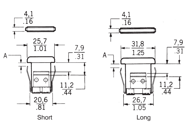
Mounting barriers
