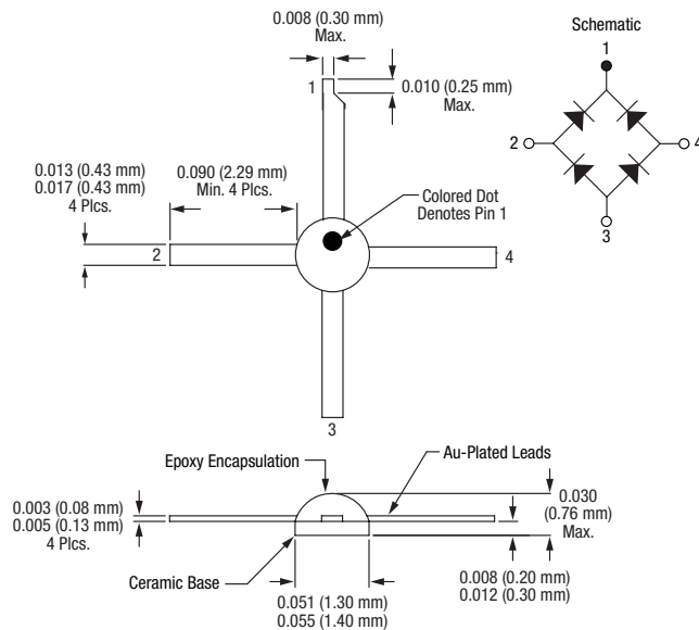
Figure 14. -235 Package Dimensions
