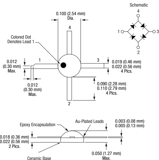
Figure 19. -254 Package Dimensions
