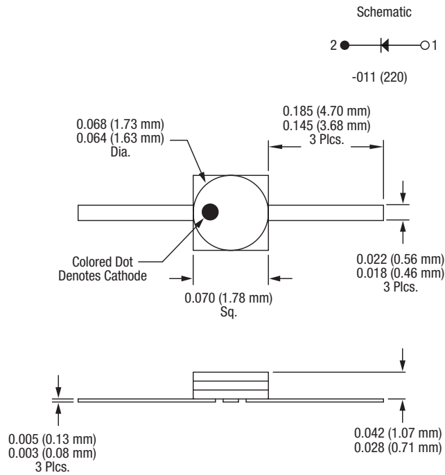
Figure 5. -220 Package Dimensions
