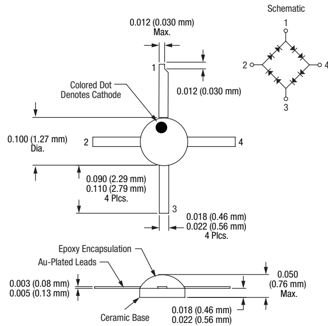
Figure 21. -257 Package Dimensions
