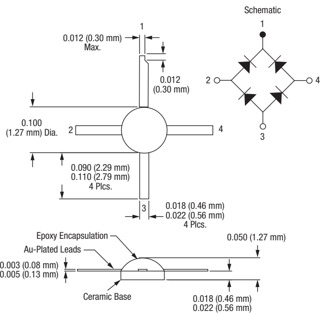
Figure 20. -255 Package Dimensions
