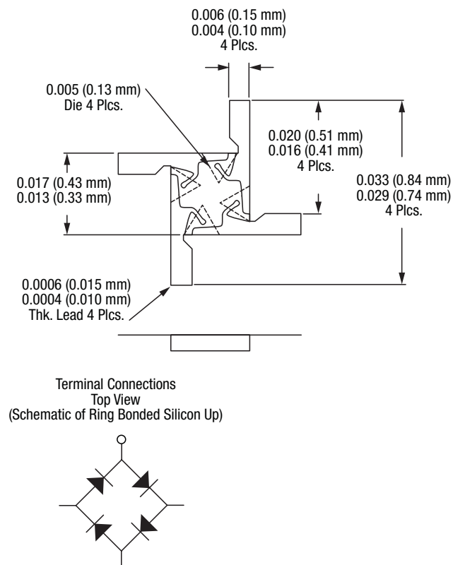
Figure 22. 488-002 Package Dimensions
