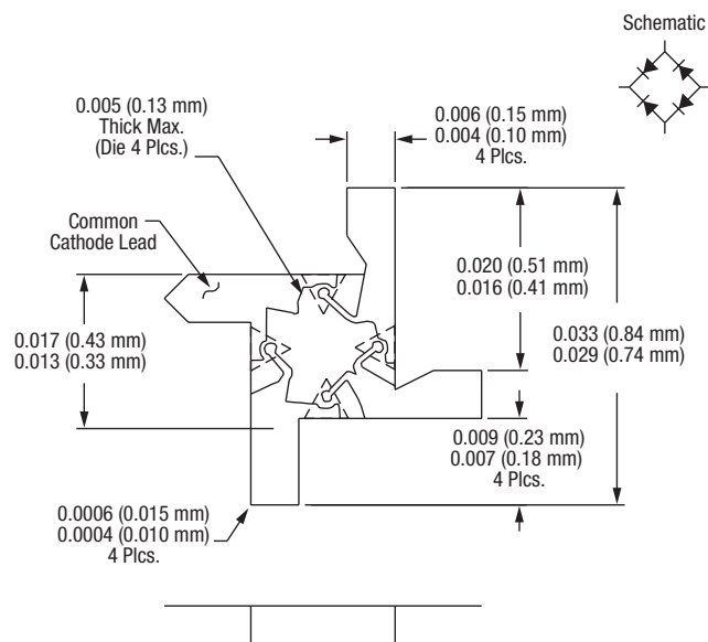
Figure 23. 488-004 Package Dimensions
