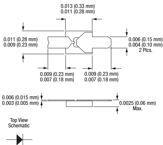
Figure 24. 491-011 Package Dimensions
