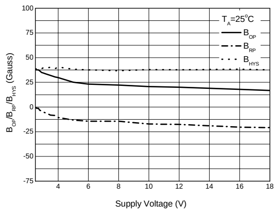
Figure 9. B_{OP}/B_{RP}/B_{HYS} vs. Supply Voltage
