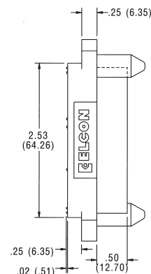
Part Number 1648163-1
