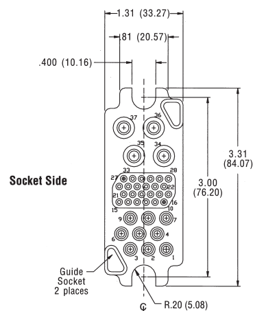
Part Number 1648162-1
