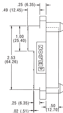
Part Number 1648162-1
