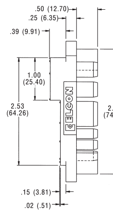
Part Number 6648167-1
