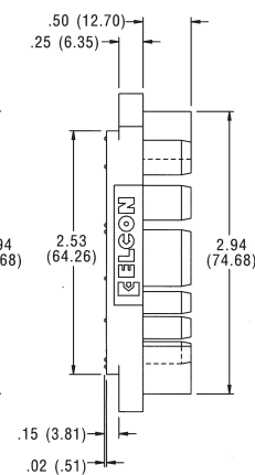
Part Number 1648168-1
