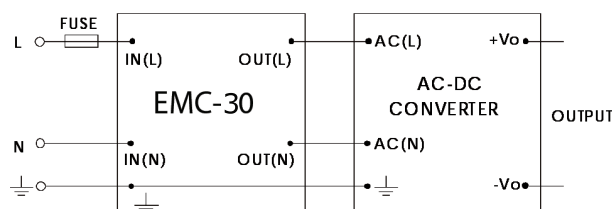
Figure 2 Application Circuit
