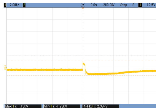
Output voltage waveform (Differential mode 0.90KV)
