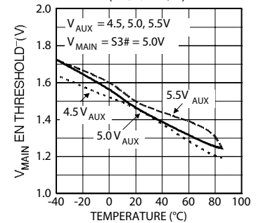
Enable Threshold (decreasing) vs. Temperature (MIC2012-1/-2)
