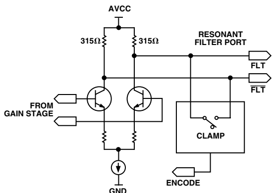
Figure 23. 4×/8× Amplifier Clamp Circuitry
