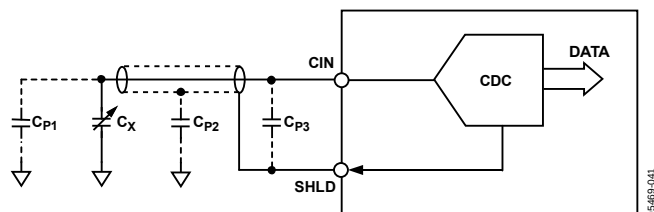
Figure 33. Parasitic Capacitance
