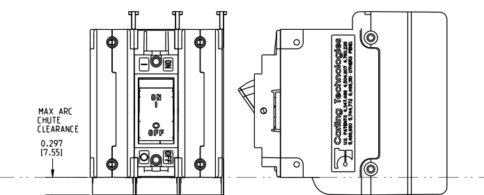
3-POLE (CF3,CG3,C13,C23) w/ ARC CHUTE BARRIER
