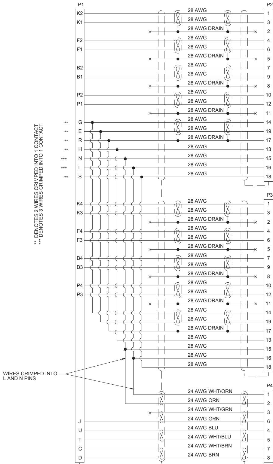
WIRING DIAGRAM
