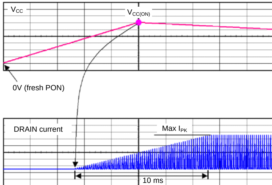
Figure 39. The 10 ms Soft-start Sequence
