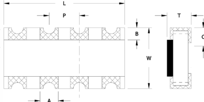
Package Drawing – Concave, Type X
