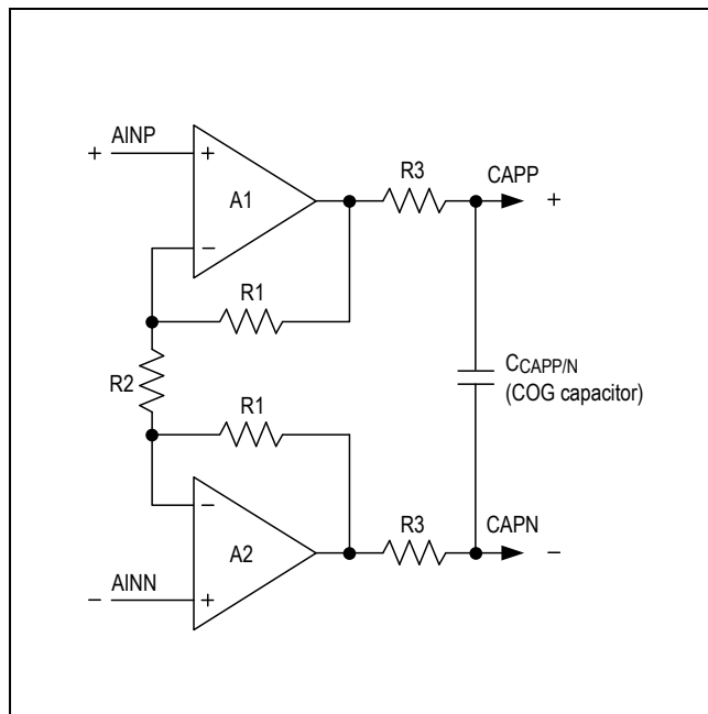
Figure 1. PGA Structure
