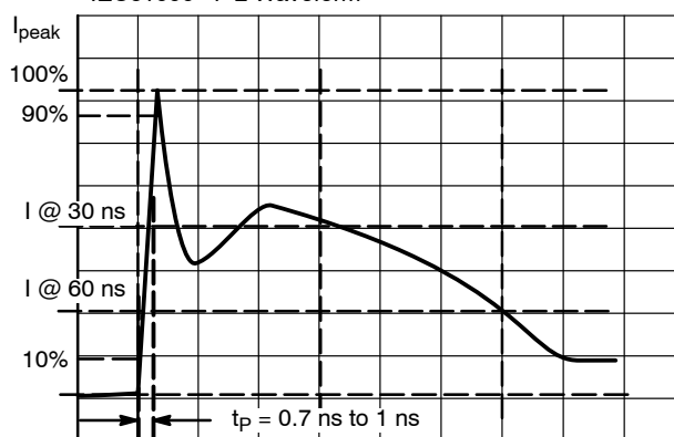
Figure 3. IEC61000-4-2 Spec
