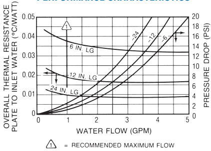
PERFORMANCE CHARACTERISTICS
