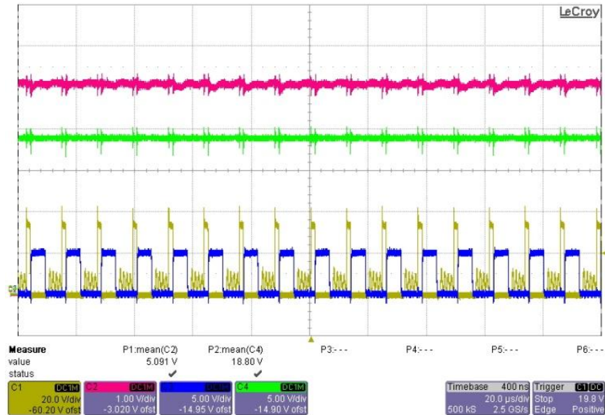
Figure 27. 264 V_{AC} , Near Over-Power Protection (CH1: DET, CH2: SR V_{DD} , CH3: SR Gate, CH4: V_{DD\_1st} )
