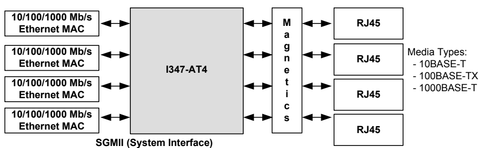
Figure 2. SGMII (System) to Copper — Quad Port Mode
